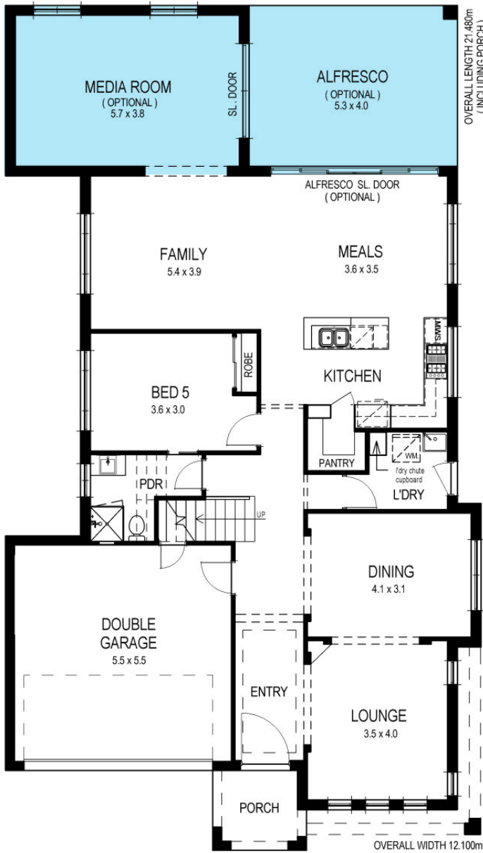
Ground Floor
