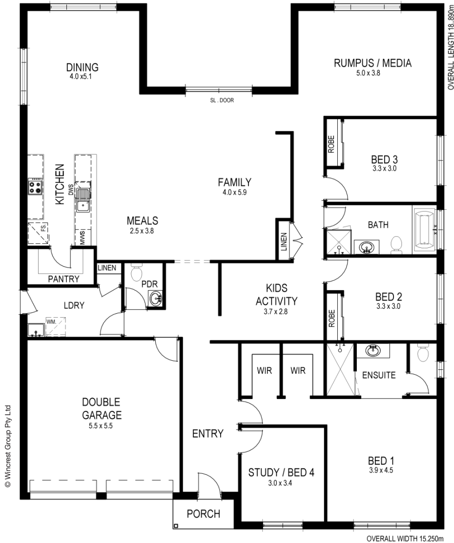
Standard floor plan as priced.
